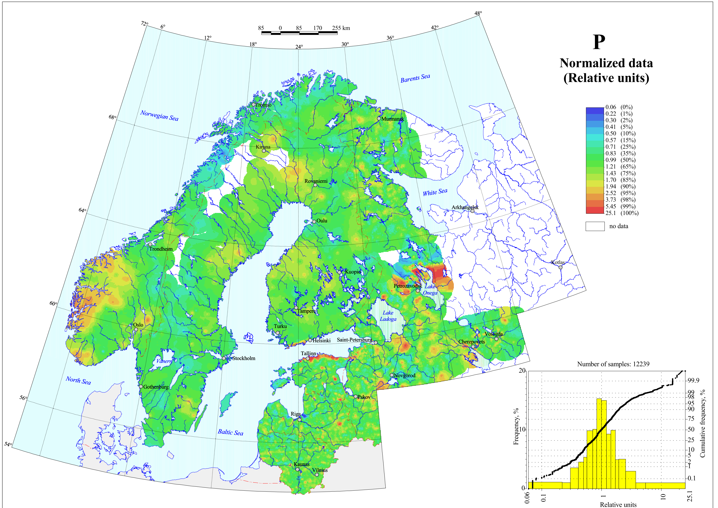
Phosphorus in Topsoil
